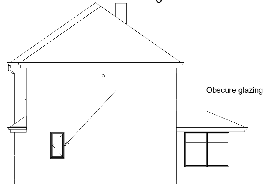
4 West elevation 1 : 100
